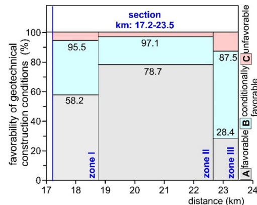
Figure 10. Terrain zoning according to geotechnical conditions for construction (km: 17.2-23.5)
